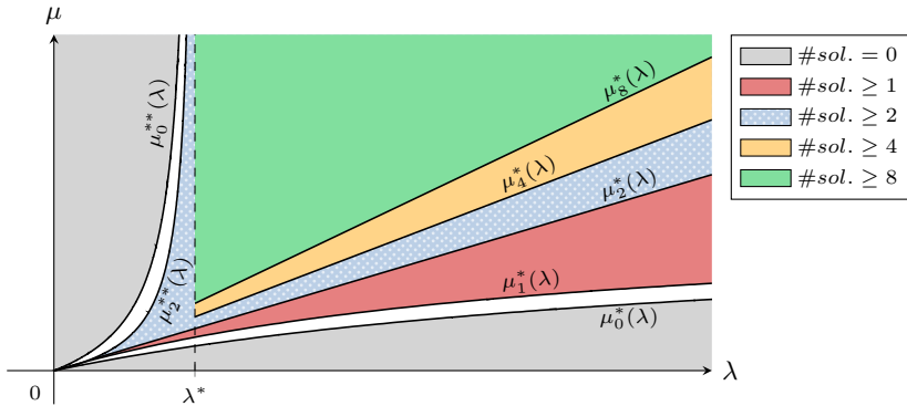
FIGURE 1. Qualitative bifurcation diagram of the solutions to (1.1) in the (\lambda, \mu) -plane. The curves \mu_0^*(\lambda) and \mu_0^{**}(\lambda) define the non-existence region (gray). The curves \mu_1^*(\lambda) and \mu_2^{**}(\lambda) mark out regions of existence: at least one solution in between \mu_1^*(\lambda) and \mu_2^*(\lambda) (red) and at least two solutions in between \mu_2^*(\lambda) and \mu_2^{**}(\lambda) (blue). For \lambda \in [\lambda^*, +\infty) , at least four solutions in the region above \mu_4^*(\lambda) (yellow), and at least eight solutions in the one above \mu_8^*(\lambda) (green).
