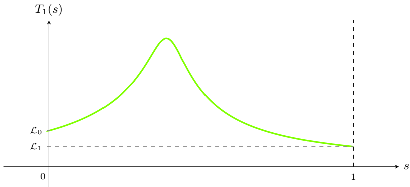
FIGURE 6. For \lambda \in (0, \lambda^*) and \mu > \tilde{\mu}(\lambda) , qualitative graph of T_1 , which is the time necessary to connect \Gamma_0 to \Gamma_1 , as a function of the initial data u(0) = s of (2.5).
