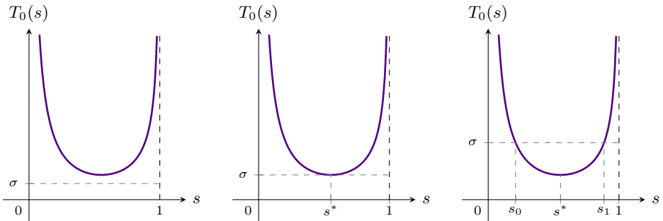
FIGURE 2. Qualitative graph of the function T_0 when \lambda \in (0, \lambda^*) (left), \lambda = \lambda^* (center), and \lambda > \lambda^* (right). The points s^* , s_0 , and s_1 are defined in Proposition 2.1.
