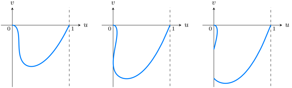
FIGURE 3. Qualitative representation in the (u, v) -plane of the curve \Gamma_0(\lambda) defined in (2.11) when \lambda \in (0, \lambda^*) (left), \lambda = \lambda^* (center), and \lambda > \lambda^* (right).
