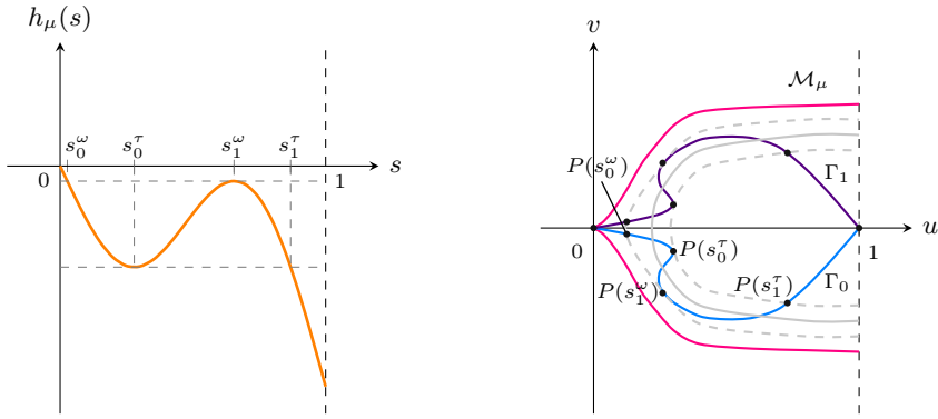
FIGURE 7. For \lambda \in (0, \lambda^*) , qualitative representations of the graph of the function h_\mu defined in (4.4) (left) and of \Gamma_0 (blue), \Gamma_1 (violet), \mathcal{M}_\mu (pink) along with some level lines of (3.2) (gray) in the (u, v) -plane (right). We set P(s) = (u_s(\sigma), v_s(\sigma)) .
