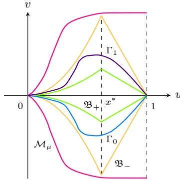
FIGURE 9. For \lambda \in (0, \lambda^*) , qualitative representation in the (u, v) -plane of the curves \Gamma_0 and \Gamma_1 , the manifold \mathcal{M}_\mu , and the curves \mathfrak{B}_- and \mathfrak{B}_+ .
