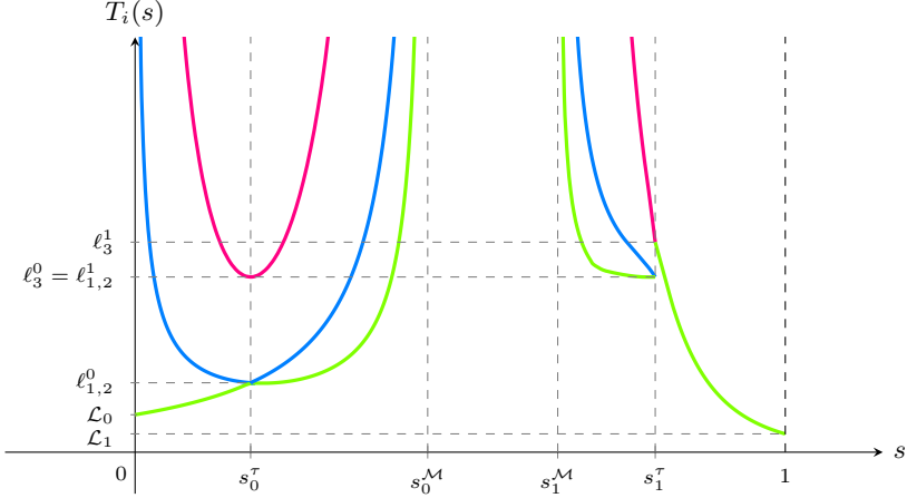
FIGURE 5. For \lambda \in [\lambda^*, +\infty) , qualitative graphs of T_i , with i = 1, 2, 3 , which are the times necessary to connect \Gamma_0 to \Gamma_1 , as functions of the initial data u(0) = s of (2.5): T_1 (green), T_2 (blue), and T_3 (pink).
