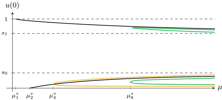
FIGURE 10. For \lambda \in [\lambda^*, +\infty) fixed, a minimal qualitative bifurcation diagram for (1.1) with \mu as bifurcation parameter. The topological configuration involves: two unbounded branches bifurcating from 0 and 1 (black) and three unbounded branches (yellow, green) originating from a supercritical pitchfork bifurcation and two supercritical turning points, respectively.
