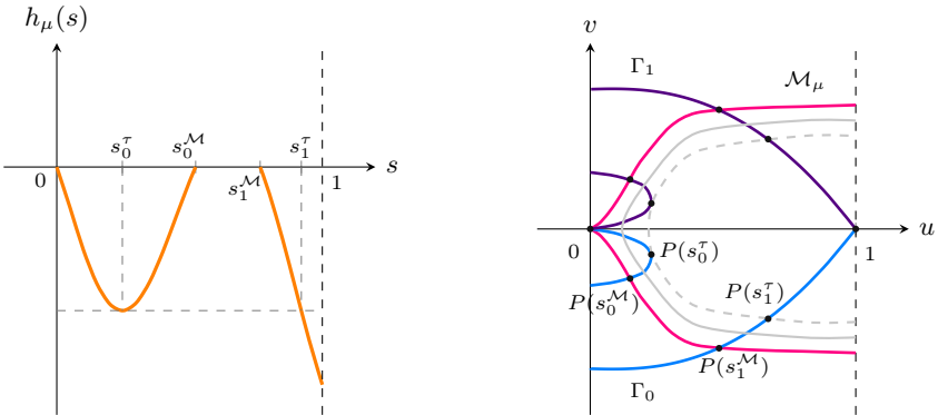
FIGURE 4. For \lambda \in [\lambda^*, +\infty) , qualitative representations of the graph of the function h_\mu defined in (4.4) (left) and of \Gamma_0 (blue), \Gamma_1 (violet), \mathcal{M}_\mu (pink) along with some level lines of (3.2) (gray) in the (u, v) -plane (right). We set P(s) = (u_s(\sigma), v_s(\sigma)) .
