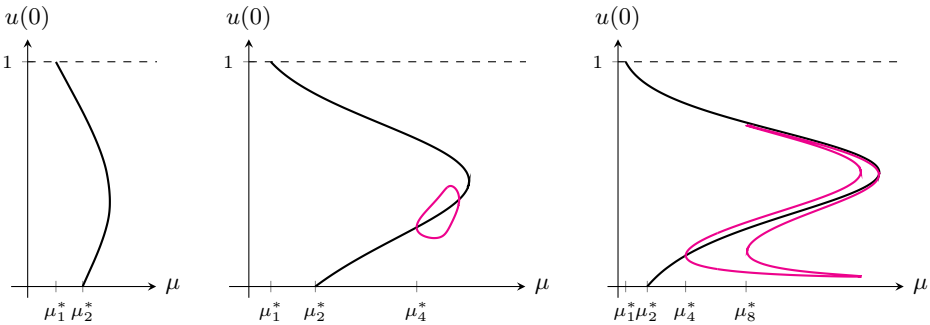
FIGURE 11. For \lambda \in (0, \lambda^*) fixed, minimal qualitative bifurcation diagrams of (1.1) with \mu as bifurcation parameter. Depending on \lambda , different topological configurations may appear: only a bounded connected branch (black) connecting 0 to 1 producing one to two solutions (left) or a connected branch crossed by a loop (magenta) which increases the number of solutions up to either four (center) or eight (right).
